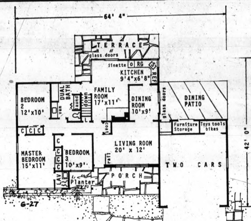
FLOOR PLAN — Study of floor plans shows that architect has used compact lay- out to include many features not ordinarily included in house with such modest dimen- sions.
