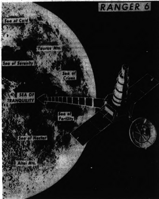
EXPECTED APPROACH — This is how the spacecraft Ranger 6 is expected to approach the moon for a crash landing into the Sea of Tranquility tomorrow. Hopefully, the
