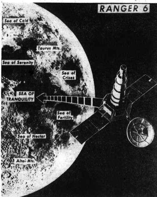
EXPECTED APPROACH — This is how the spacecraft Ranger 6 is expected to approach the moon for a crash landing into the Sea of Tranquility tomorrow. Hopefully, the spacecraft's TV camera will transmit pictures until the moment of impact. The Sea of Tranquility is a great flat basin, roughly comparable to California's Death Valley.
