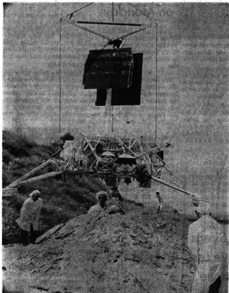
MODEL 'MOON' LANDING —A model of the Surveyor 4 spacecraft, which will attempt a gentle touch-down on the moon, goes through tests by engineers at Hughes Aircraft Co. in Los Angeles. The latest Surveyor will carry a new tool—a tiny magnet—to determine whether the lunar soil contains magnetic particles. The Hughes firm builds Surveyors for NASA.
