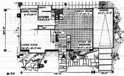
FLOOR PLAN — Attached garage makes possible full use of grade level for living space
