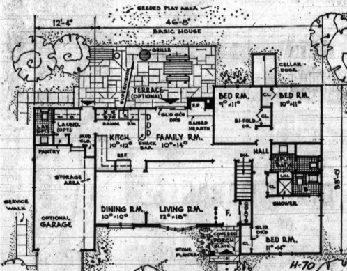
FLOOR PLANS —A lot of thought obviously went into Design H-70, evidenced by the excellent traffic pattern, separating the living, service and sleeping areas and giving free movement without using the living and dining rooms as passageways.
