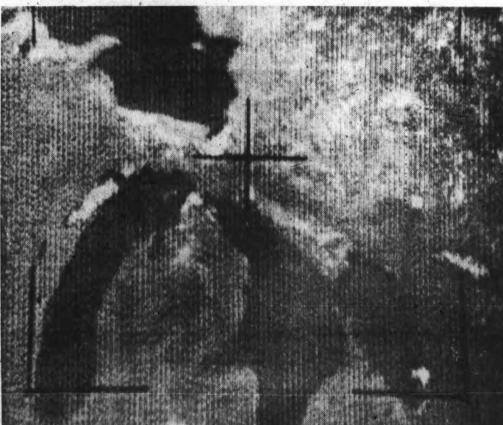
TIRES PICTURE — This photograph shows Michigan as it looks from 400 miles in space. The picture was taken by Tires IV, one of the United States' weather satellites. The picture was received at Wallops Island, Va., while a group of Michigan officials was on tour. A copy of the photo was given to each of them.
