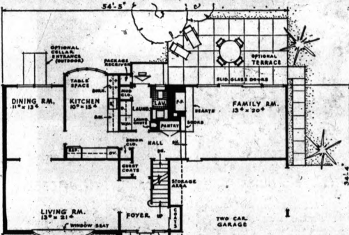
TRADITIONAL PLUS: Basic features of Early American house, which has been given a fresh character by modern architecture are retained in this four-bedroom, two-story design touches and materials.
