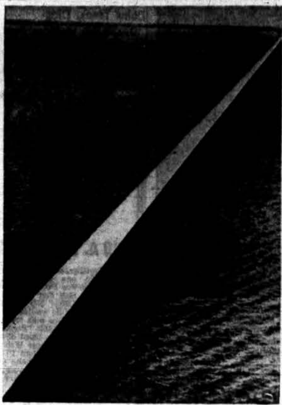
LONG BRIDGE READY FOR OPENING —The Lake Pontchartrain Causeway, New Orleans, La., a two-lane concrete bridge extending 28.83 miles across the lake from north to south, will be opened today. This longest overwater highway bridge was built in 15 months at a cost of $6 million dollars. Toll for a passenger automobile is one dollar.
