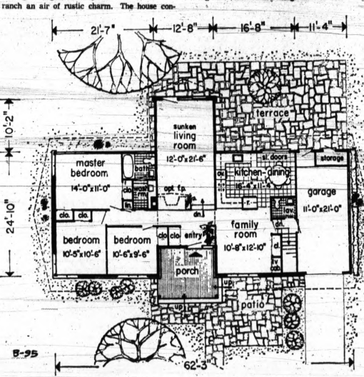
FLOOR PLAN —Shape of this house is unusual, but consists of simple rectangular forms which permit framing system. Stone fireplace in living room is optional feature. If built, boiler flue would be inside chimney, and vanity in wash room lengthened. Note efficient plan of kitchen.
