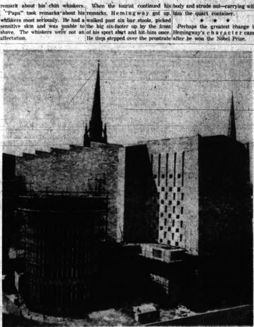
RISE IN ANEW — Construction scaffolding has been removed from the zigzag walls of the nave of Coventry Cathedral in Coventry, England. The church is being built on the site of the 14th century building which was destroyed during World War II by German bombings. Structure at left is an almost completed guild chapel. In background are spires of St. Michael Cathedral.
