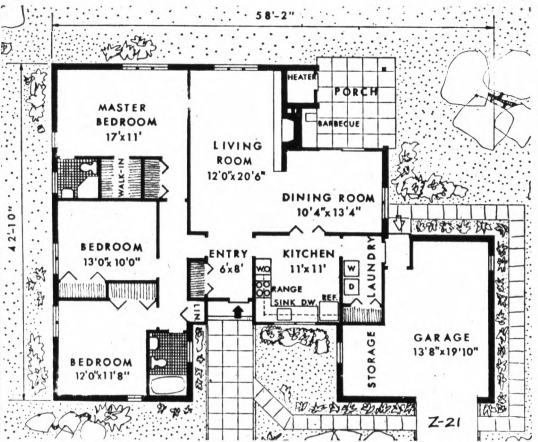
FLOOR PLANS —Maximum utilization of all available space is clearly evident. Entry foyer is hub of circulation pattern. Open
