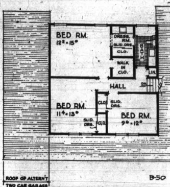
BEDROOM LEVEL —Master bedroom is large and equipped both with walk-in closet and a dressing room which leads to main bath.
