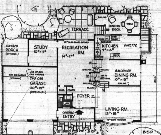
LOWER LEVELS —Recessed entry provides practical shelter for the trip from front door to garage. There is a choice of routes to the upper level, either from the foyer or from recreation room.
