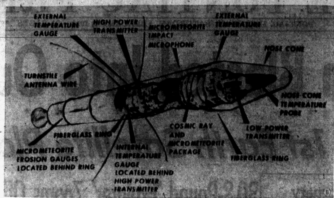
DIAGRAM OF SATELLITE — This cutaway diagram showing instruments contained in the U. S. Army earth satellite was released in Washington today by the Defense Department. The satellite, christened "Explorer" by the department, was propelled into orbit around the earth by the Army's Jupiter-C missile last night.
