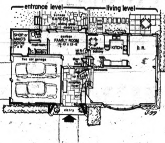
STATELY SPLIT — This nine-room split level has four bedrooms, 2½ baths and an exceptionally efficient floor plan. The attractively accented entrance is on grade level, adding space and privacy to the living room.
