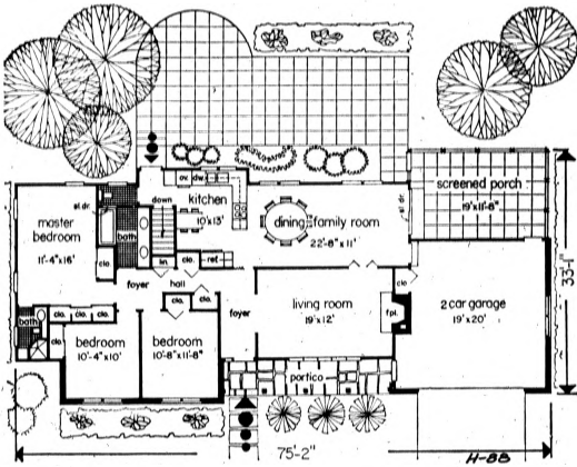
FLOOR PLANS: The 1474 square feet of living area in this three-bedroom ranch house are divided into specific zones, yet have the kind of open effects which are so marvelous when extra space is needed for entertaining.
