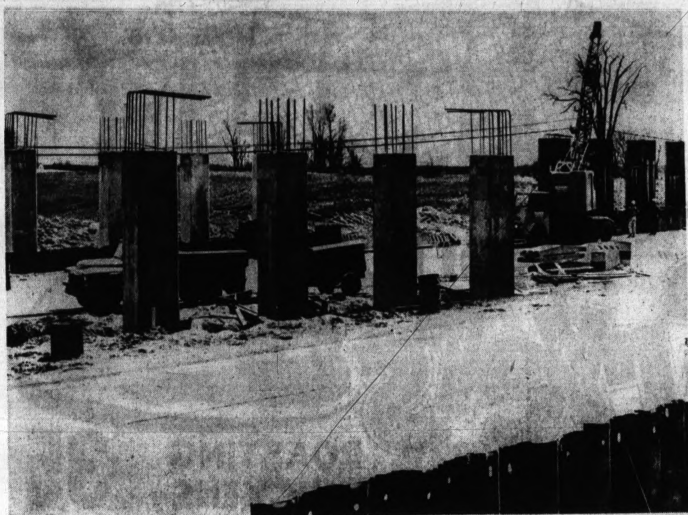
BIRTH OF AN EXPRESSWAY — Have you driven off M24 (Lapeer Road) lately on the way from Pontiac to Lake Orion or Oxford? If you have, you have seen these structures, known to engineers as pier columns. The first section you'll see represents the main crossing where the Walter P. Chrysler Expressway will
