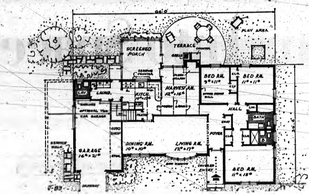
FLOOR PLAN —House contains 1,417 square feet of living area not counting the 280-square foot garage. If desired, garage could be widened to two-car size. Living room bow window is floor-to-ceiling; screened porch has translucent plastic roof.
