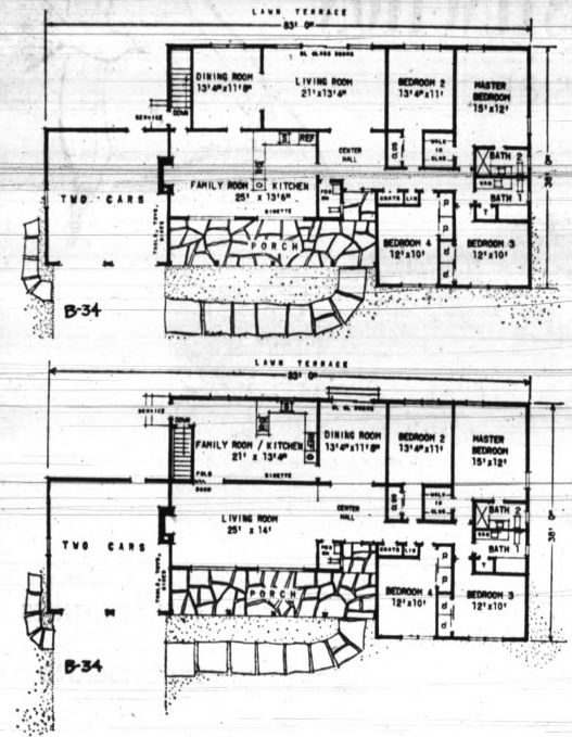
AS YOU LIKE IT — The two floor plans above are for the same house. The design includes an option on division of space in the living section. You can locate living room in back with kitchen in front, or kitchen in back with living room in front.
