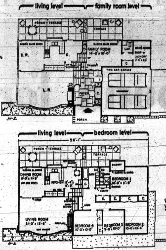
FLOOR PLANS — The living and bedroom levels contain 1,553 square feet including the porch. The family room level, not including the garage, adds 433 square feet of bonus space. Overall dimensions are 30 feet 8 inches deep by 56 feet 1 inch wide.
