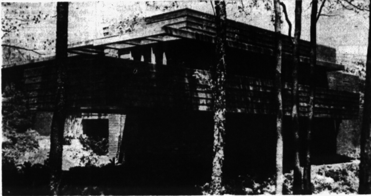
CANTILEVERS PART OF WRIGHT PLAN — Brick columns support cypress framed cantilevers in the Gregor Affleck home designed by Frank Lloyd Wright. The long balcony facility is accessible from the second level combination living-dining room and is an outdoor living room and porch. In a heavily wooded area, an abundance of shade is provided in the summer months.
