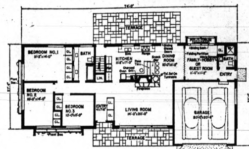
FLOOR PLAN —Four exterior entrances guarantee excellent traffic movement in and out of this house. Note the abundance of closet space in the entry, family room and hallway as well as the bedrooms. House has a full basement which can be partitioned as the owner desires.
