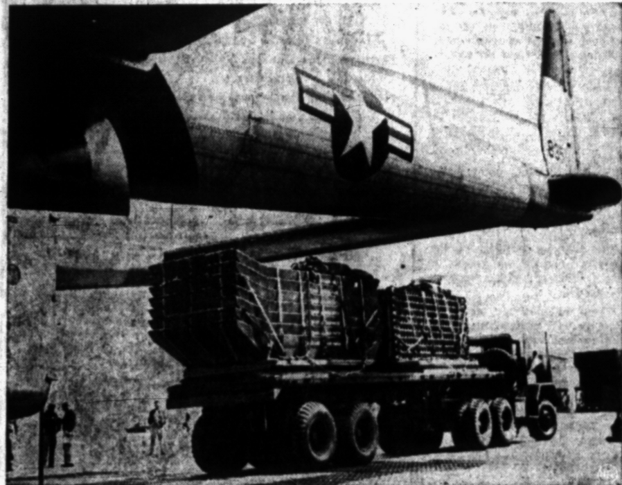
A truck carrying part of the 474-foot aluminum bridge rolls up to a Flying Boxcar which will drop the span for a troop-training mission.
