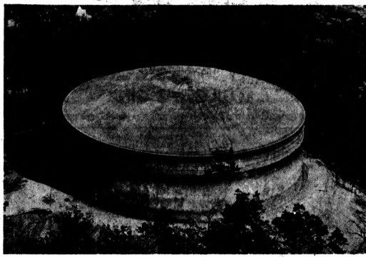
Aerial View Of Waterford's 6-Million-Gallon Water Tank
