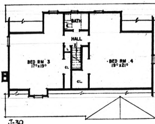
J-30 UPPER FLOOR PLAN
