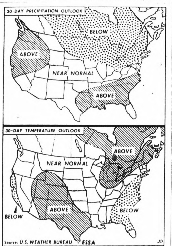
30-DAY FORECAST — The weather in the Pontiac area over the next 30 days will include above-normal temperatures and below-normal precipitation, according to these charts released today by the U.S. Weather Bureau.
