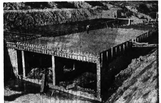
BIG DRAIN — Much of the basic design of the 12-Towns Relief Drain, shown here in the construction phase several years ago, were handled by Hubbell, Roth & Clark Inc. of Bloomfield Township. The system provides storm water relief for 12 communities encompassing 24,500 acres in Oakland County
