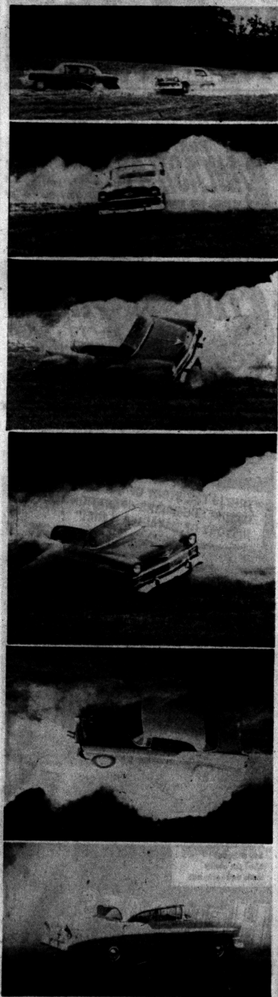
OVER AND UP — The only way to test what will happen if a car rolls over at high speed is to roll one over. So, technicians at the General Motors Proving Ground at Milford hooked this car, minus driver, behind another and towed it into the open. Some preset mechanisms took over and the car rolled over and up on its wheels, demonstrating the sturdiness of the car but not necessarily assuring that all cars will come back up on the wheels after a similar rolling journey.
