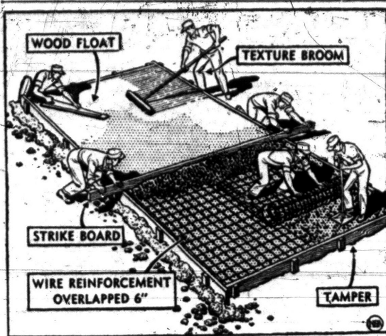
POURING A CONCRETE DRIVEWAY —This composite drawing of concrete driveway construction shows all steps at once. Remember, however, each step must be completed before the next is begun.
