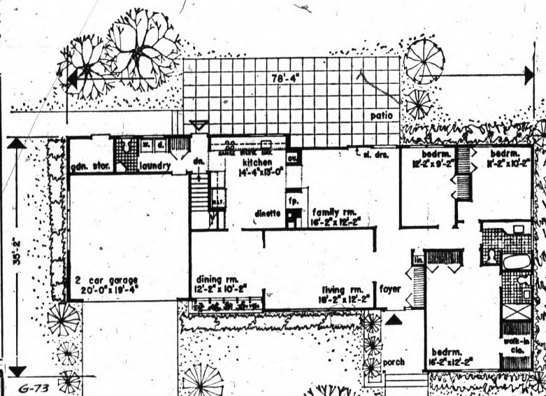
FLOOR PLANS: The 1660 square feet of living space in this three-bedroom ranch have been made to seem much larger by the excellent floor layout, which puts the living room and dining room, as well as the kitchen and family room, in a side-by-side alignment.
