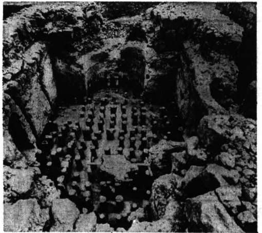
The caladrium, or hot room, of a large bath house. Hot air was piped between pillars shown, heating the floor above.
