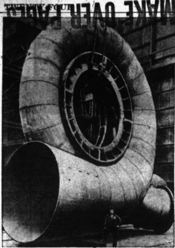
BRITAIN'S INDUSTRY BOOMS — This huge, horn-like spiral casing in London, England, will house plenty when filled with a 73,000-horsepower water turbine and shipped to Portugal. The 35-foot-high, 66-ton casing dwarfs the man at bottom of photo. Great Britain is in the midst of a new industrial export boom.
