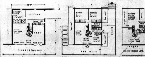
FLOOR PLANS: Utilizing all three floors of this A-frame, the architect has provided everything necessary for comfortable living for a family needing three bedrooms, but the lower and upper levels need only be roughed in if not immediately needed.
