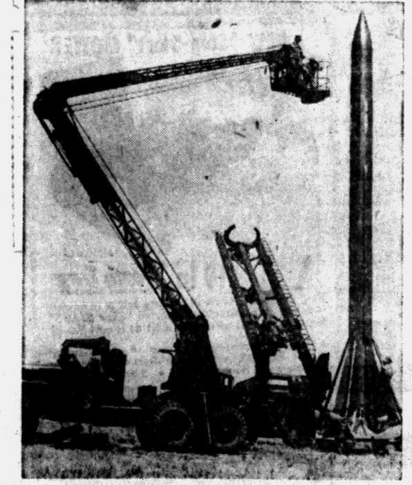
system of the "Corporal" rocket at the U. S. Army Ordnance Guided RIDING HIGH — Two students get a big lift in what GI's call a "cherry picker," a huge boom which provides access to the control Missile School, Fort Bliss, Tex. An erector (center) stands the rocket on its launcher.
