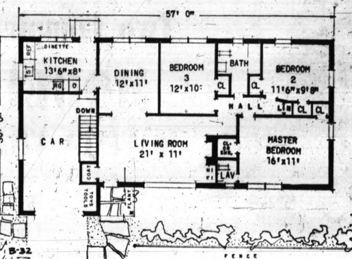
FLOOR PLAN —Living room is extra large and leads into a full-fledged dining room.
