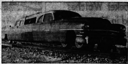
THE BLUE GOOSE EXPRESS — Two-thirds automobile and one-third locomotive, a unique vehicle transports personnel between a gypsum plant and quarry at Plaster City, Calif. Dubbed the Blue Goose, the 34-foot-long, 6,000-pound rail car rides along at 40 m.p.h. on eight steel-cord tires with flanges at-
