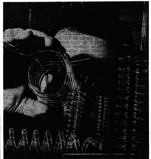
Inspecting glass coil (made by winding heated tube around asbestos-covered rod).
