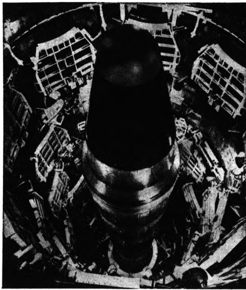
Resting in its 150-foot shaft, topped by a nuclear warhead, is the 103-foot-tall missile.
