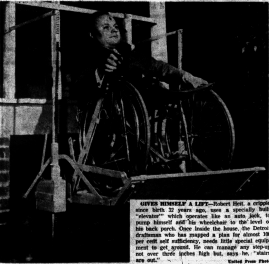
GIVES HIMSELF A LIFT—Robert Heit, a cripple since birth 32 years ago, uses a specially built "elevator" which operates like an auto jack, to pump himself and his wheelchair to the level of his back porch. Once inside the house, the Detroit draftsman who has mapped a plan for almost 100 per cent self sufficiency, needs little special equipment to get around. He can manage any step-up not over three inches high but, says he, "stairs are out."
