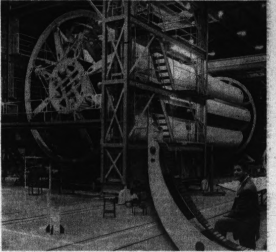
FIRST STAGE —David Campbell, project engineer for Progressive Welder and Machine Co., of Pontiac, is dwarfed by the huge first stage of the Saturn rocket. Campbell, of 4930 Big Oak Trail, Birmingham, is shown looking over the giant rocket while it was being assembled at Huntsville, Ala. The huge rings at either end, braces and framework under the rocket (partly hidden) were designed and fabricated in Pontiac. The Saturn, largest space vehicle ever built in the U.S., towers higher than a 15-story building.
