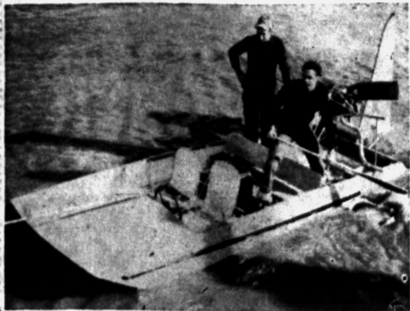
NON-FLYING AIRBOAT —Jim Hath, of Leavenworth, Kan., paddles the airboat he built out into the Missouri River for a test run, as Manuel Kuchda looks on. The 18-foot, flat-bottom craft is powered by a 75-hp. airplane engine which turns a five-foot propeller. Called the "Rushin' Henry," the craft weighs 800 pounds and is guided by air rudder at stern.
