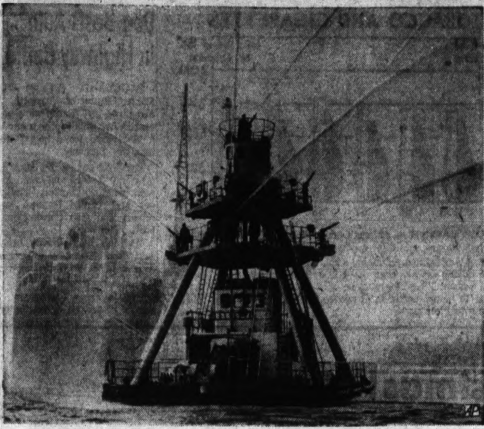
OVER-ALL COVERAGE —Water spews from the nine monitors of the British firemaster during the demonstration of new craft at Swansea, Wales. Firefighter's 40-foot-high control tower is mounted on pontoons with diesel engines fore and aft.
