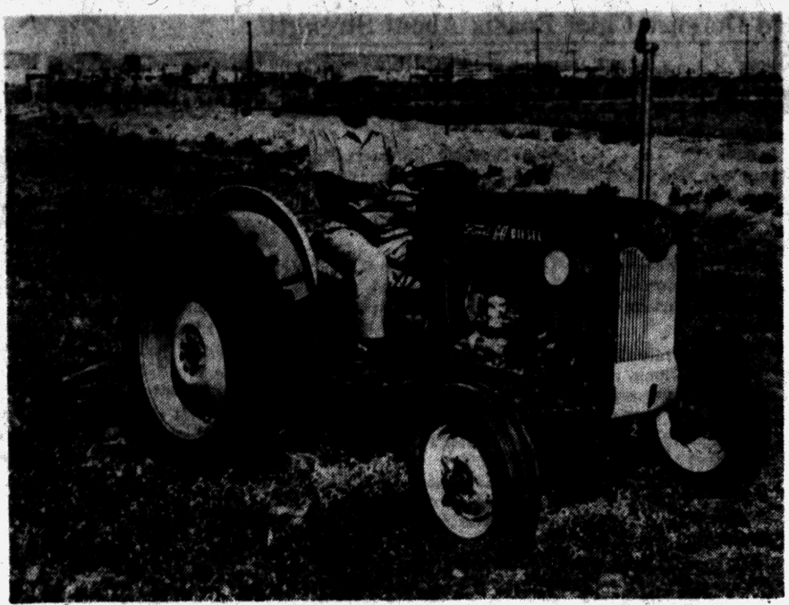
NEW FORD TRACTOR — The Ford Motor Co. has introduced this diesel tractor which is identical with the Ford Workmaster tractor in all respects except fuel requirements. Its engine has a displacement of 144 cubic inches, and a compression ratio of 16.8 to 1. The new Ford diesel is designed for fuel economy while providing sufficient power for most farm and industrial requirements.
