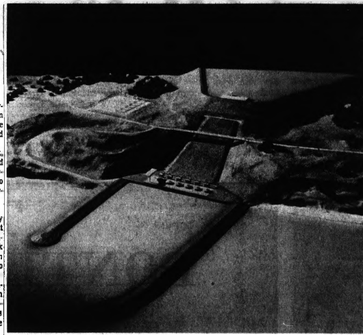
PROPOSED PLANT — This is a model of a new Consumers Power Co. pumped storage project to be built on Lake Michigan. Shown here are the upper reservoir (top) and covered penstocks with access road crossing over, and power plant at the edge of Lake Michigan. The structures reaching out into the lake (bottom) are a breakwater (left) and jetty. Construction of the plant will be partly financed by Detroit Edison Co.
