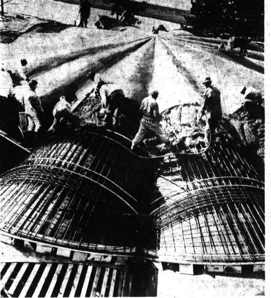
ROOF POURING PARTY —Officials and friends of the GMTC Employees Federal Credit Union yesterday held one of the most unique parties in history. They had soft drinks and doughnuts while they watched a group of workmen pour and spread 150 tons of concrete to form the roof of the modern circular wing of the new $400,000 credit union building on Woodward avenue across from St. Joseph Mercy Hospital. When finished, the roof, with a 90-foot diameter, had a thickness of 4 inches. The entire building is scheduled for completion in January.
