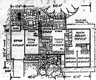
NEW DESIGN IDEAS: — The needs of a family with a limited budget dictated the unusual design of this house, a "modified ranch" with seven rooms (three bedrooms) in 1,297 square feet. A second level beneath the bedroom area, however, provides 630 square feet of additional room suitable for a variety of purposes.
