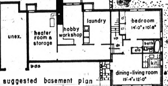
suggested basement plan
