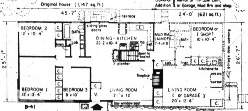
FLOOR PLAN — Heavy lines show basic section of the house; light lines indicate optional expansion.
