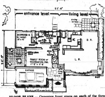
FLOOR PLANS—Generous foyer space on each of the three levels insures good traffic flow. With a small amount of alteration, entrance level could be converted into a rental apartment.
