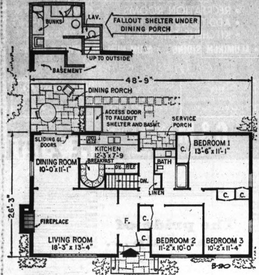
FLOOR PLAN: Inset shows location of fallout shelter beneath rear dining terrace and adjacent to basement. Living area of house, not counting full basement or shelter, contains 1,231 square feet. Above ground dimensions are 26'3" deep by 48'9" wide.
