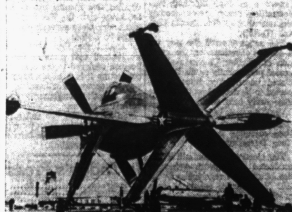
FOUR-POINT LANDING—The Navy's XFV-1, an experimental fighter made by Lockheed, which can take off and land vertically, is shown in a "four-point" position as it rests on its auxiliary landing gear during special test operations. Being capable of taking-off and landing vertically, the plane will not need runways or carrier decks on which to operate.
