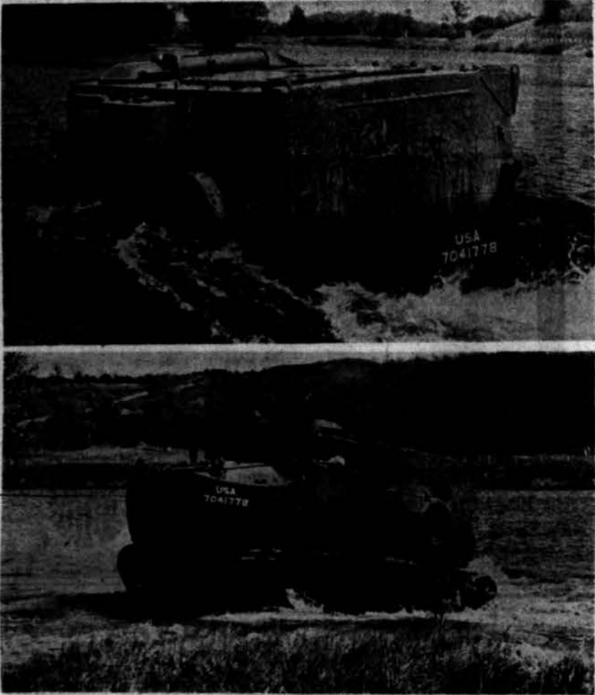
WATER BABY — The Otter, a product of Pontiac Motor Division's war production program, is an amphibious cargo carrier at home on land or in the water. Here it splashes about gaily like its namesake does in Michigan's north woods.
