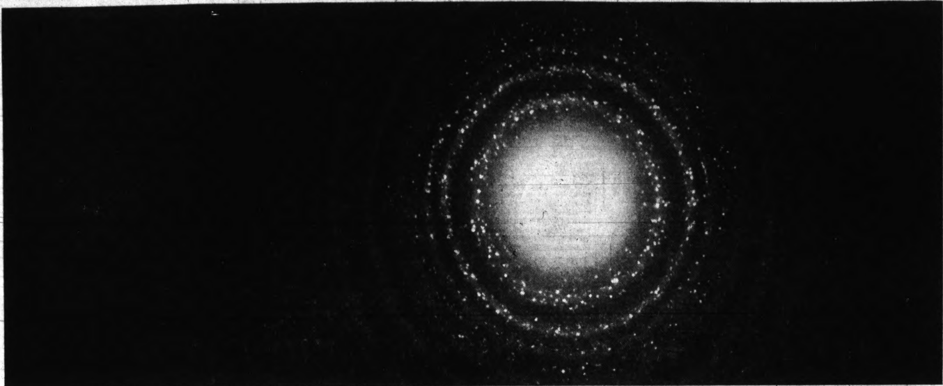
Circular pattern identifies deposits scraped from combustion chamber. It tells researchers many secrets. To get this pattern, deposits are ground up and placed above a film. Electrons are beamed directly at the deposits. The
